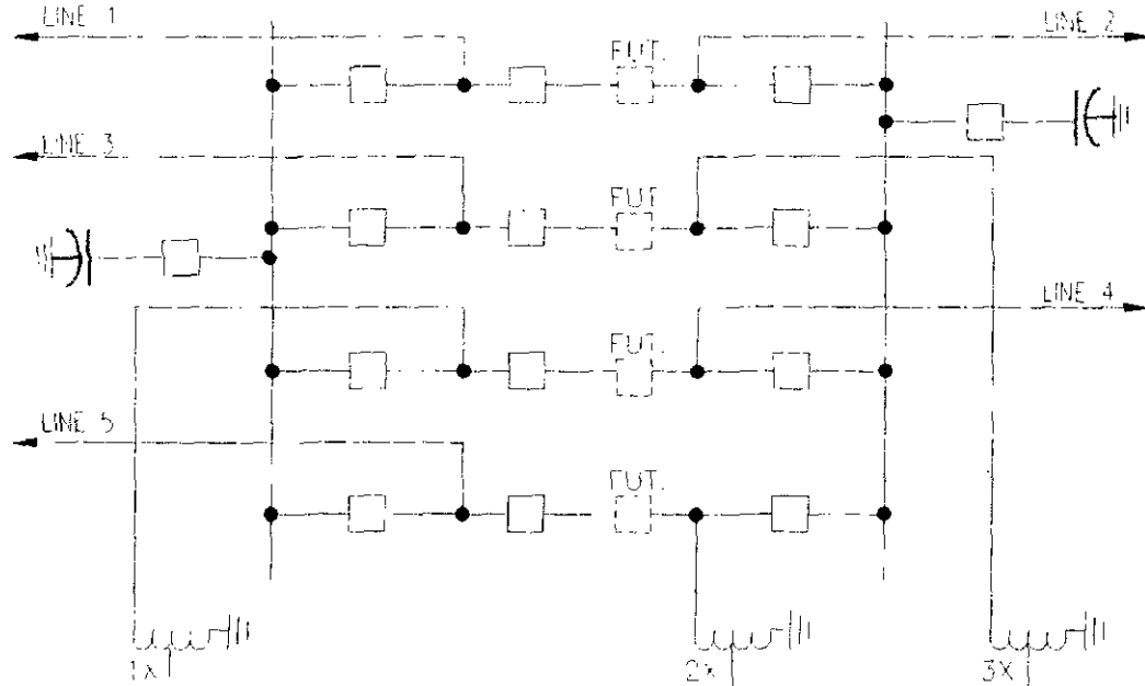
345KV BREAKER AND A HALF ARRANGEMENT (ULTIMATE)
