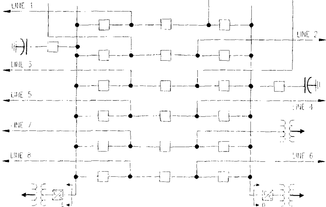
115KV BREAKER AND A HALF ARRANGEMENT (ULTIMATE)
